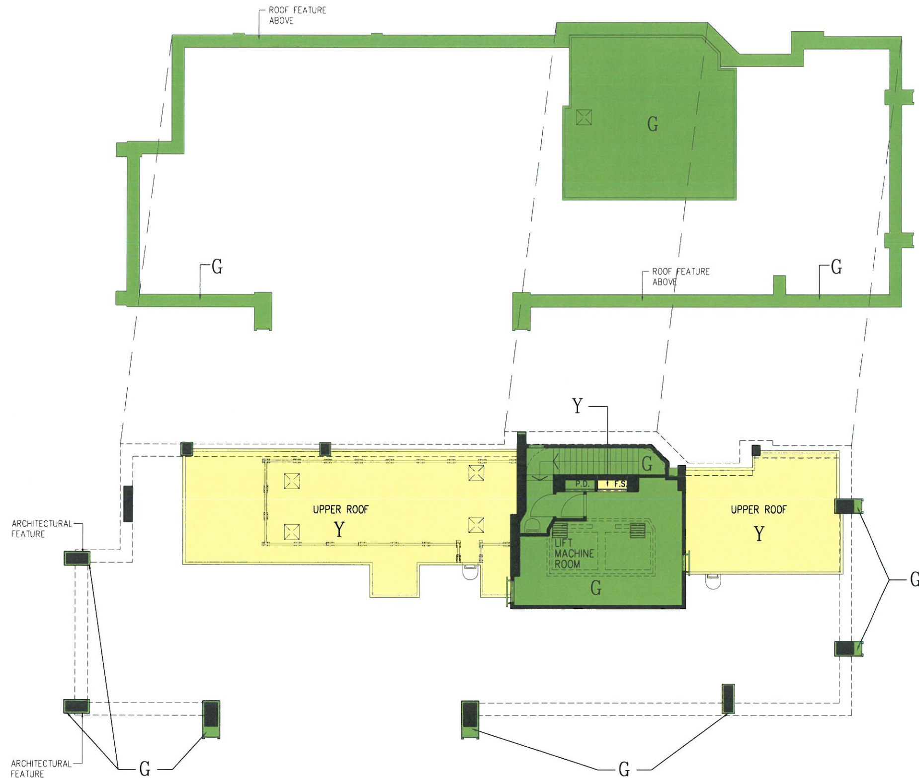
TOP ROOF PLAN
